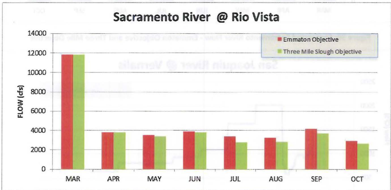
Figure 33: Forecasted DSM2 Sacramento River Flow at Rio Vista - Emmaton Objective and Three Mile Objective
