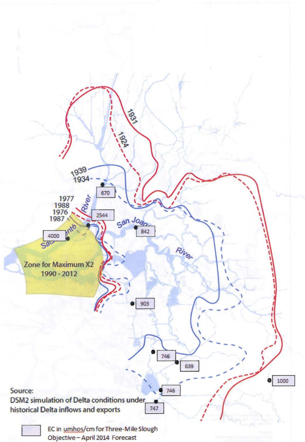
Figure 6: DSM2 Dry Years Maximum Salinity Intrusion, X2 (2640 umhos/cm)
