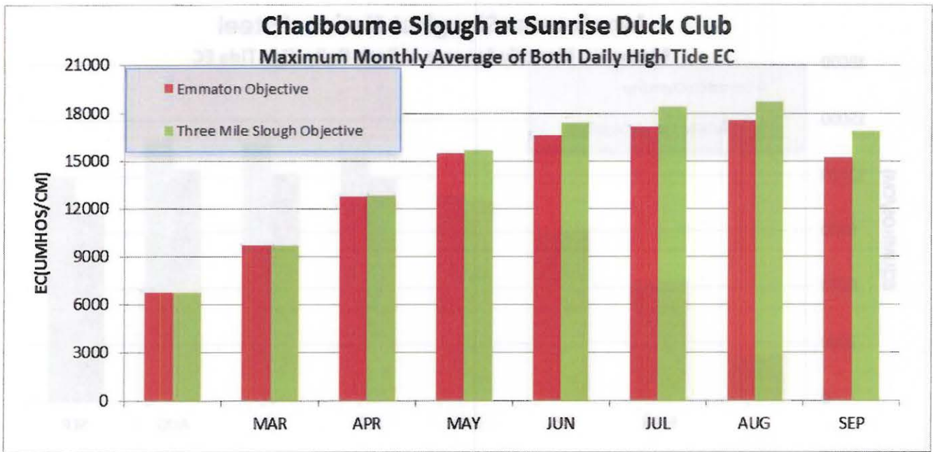
Figure 28: Forecasted DSM2 Chadbourne Slough at Sunrise Duck Club EC - Emmaton Objective and Three Mile Objective
