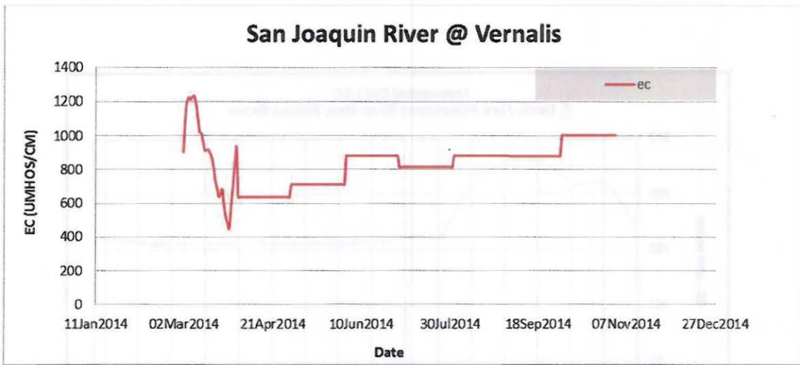
Figure 24: Forecasted San Joaquin River EC
