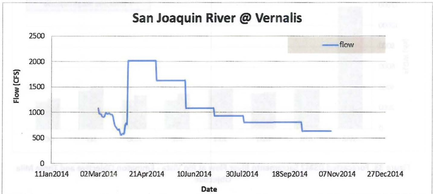
Figure 31: Forecasted San Joaquin River Flow
