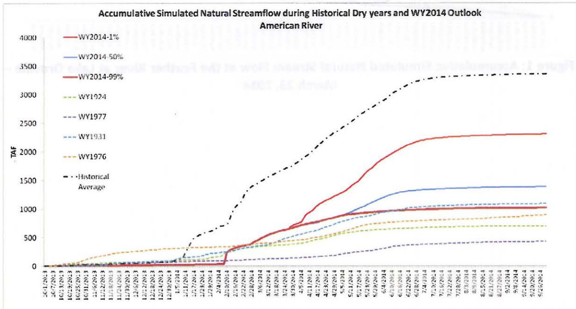
Figure 3: Accumulative Simulated Natural Streamflow at the American River- March 23, 2014
