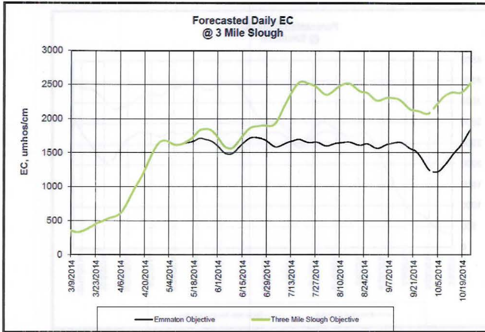
Figure 5: Three Mile Slough EC - Emmaton Objective and Three Mile Objective
