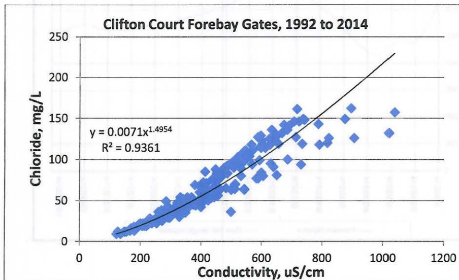
Figure 1: Chloride Correlation to EC
