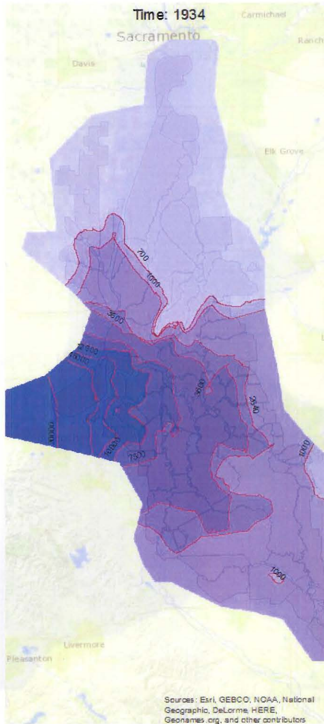
Figure 10: DSM2 1934 Maximum Salinity Intrusion, EC
