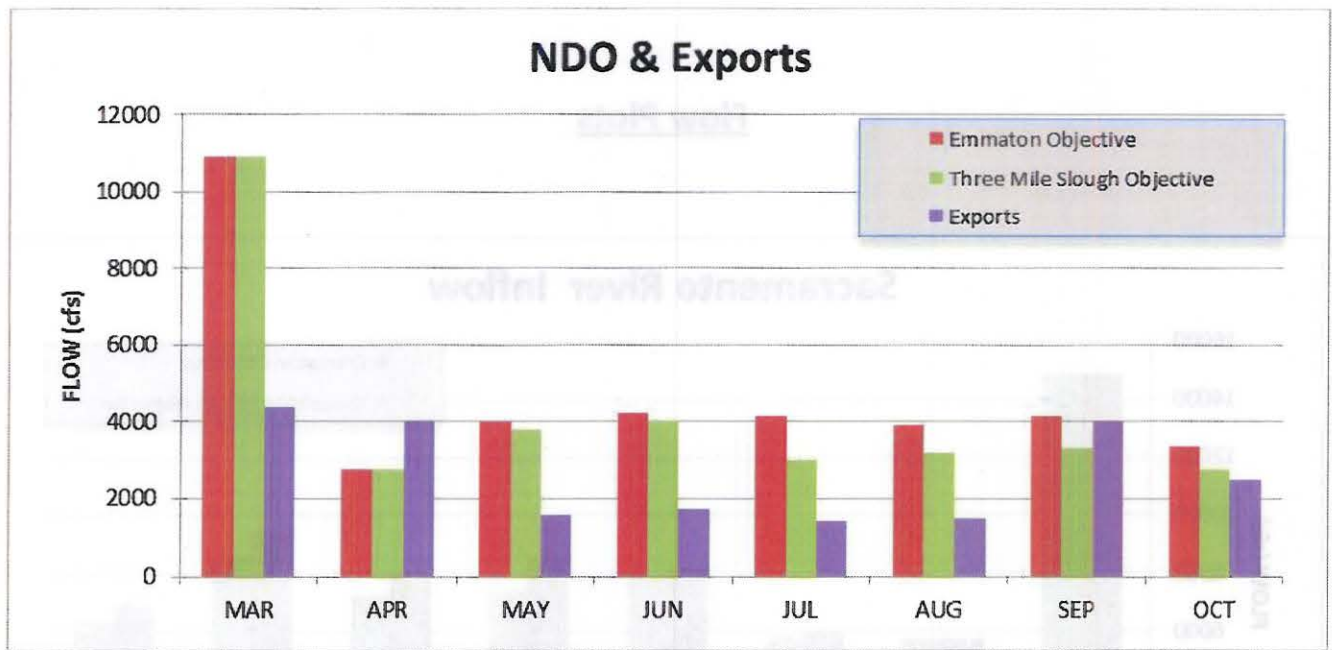
Figure 32: Exports and Net Delta Outflow with Emmaton Objective and Three Mile Objective
